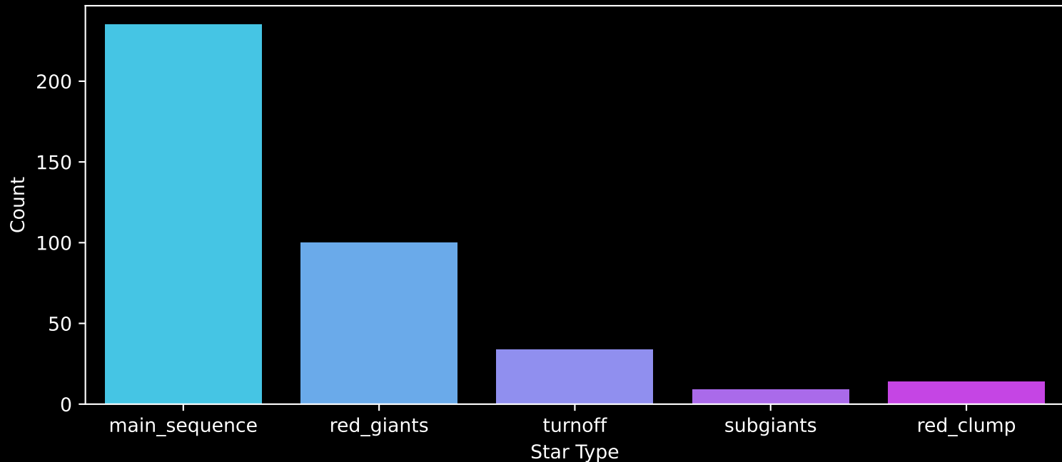
APOGEE DR17 Field: [000+60] Count plot of Star Type
