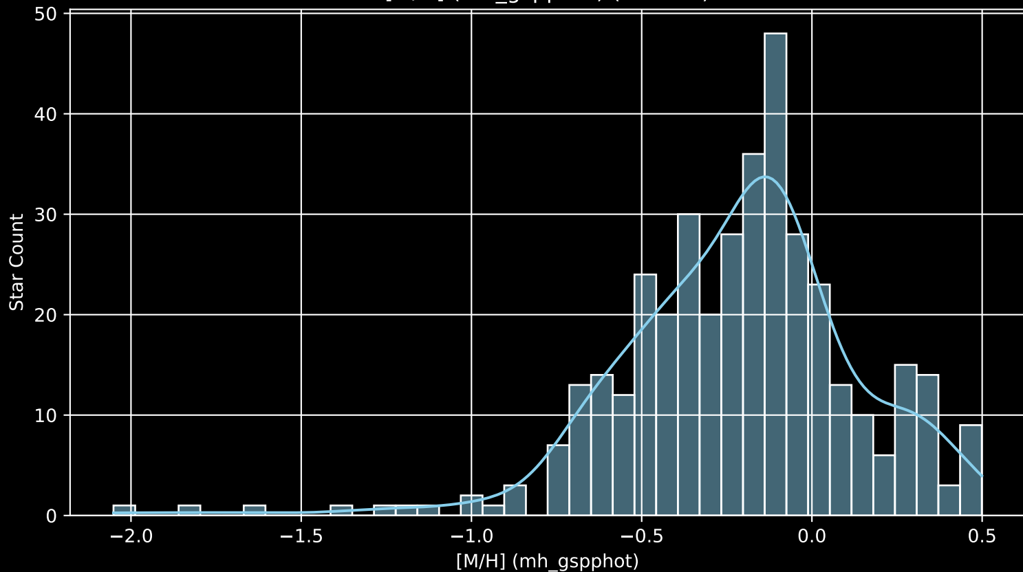
APOGEE DR17 Field: [000+60 [M/H] (mh_gspphot) (n= 386)
