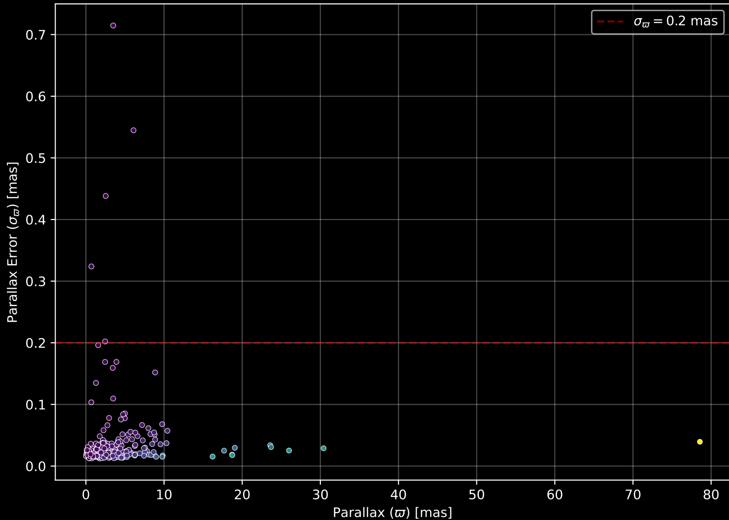
APOGEE DR17 Field: [000+60] Parallax Quality (n= 392)
