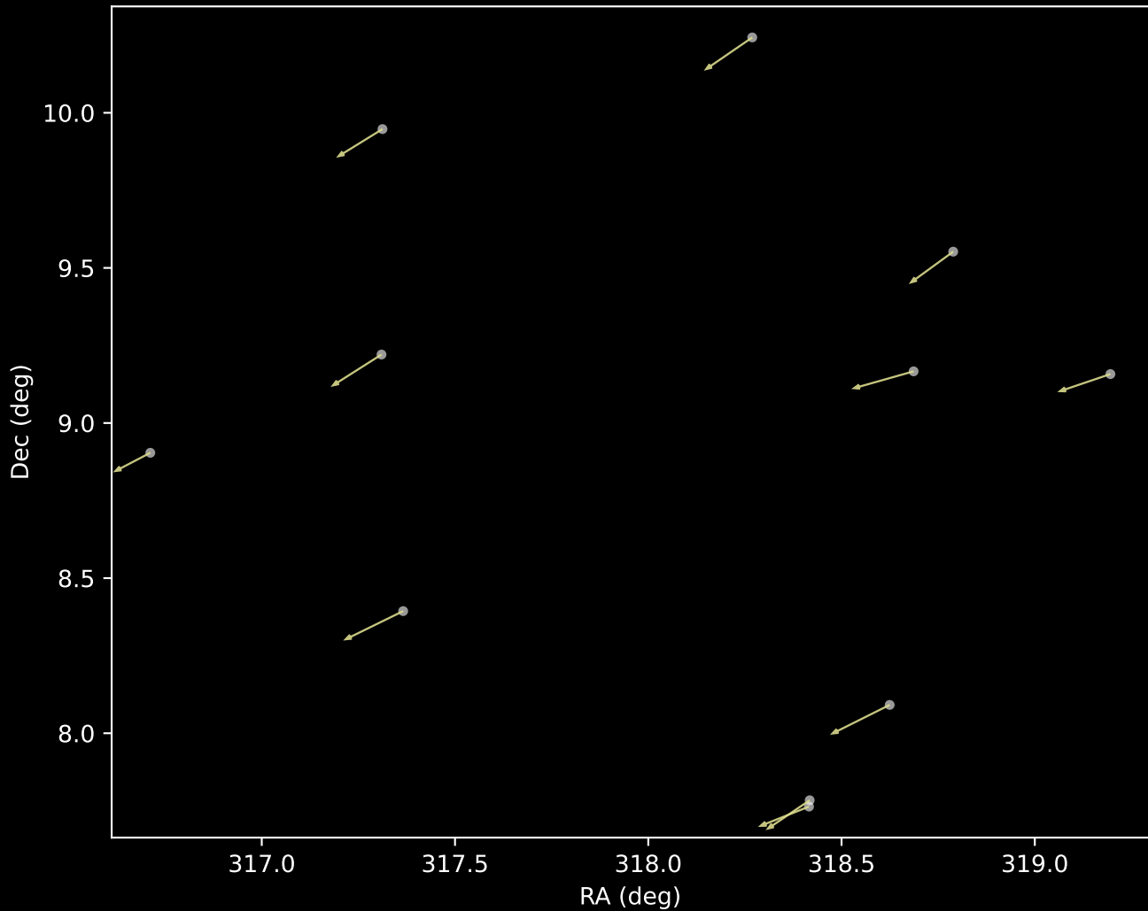
APOGEE DR17 Cluster 17 Proper Motion Vectors (n=11)
