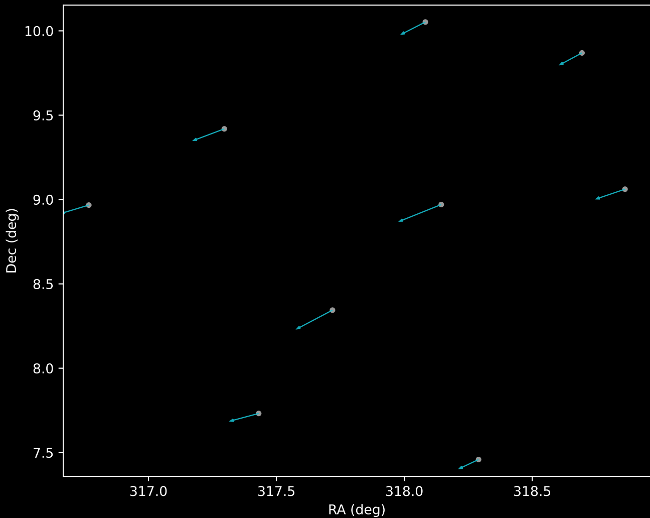
APOGEE DR17 Cluster 18 Proper Motion Vectors (n=9)
