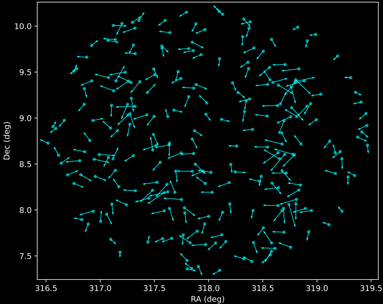
APOGEE DR17 Noise Stream Proper Motion Vectors (n=240)
