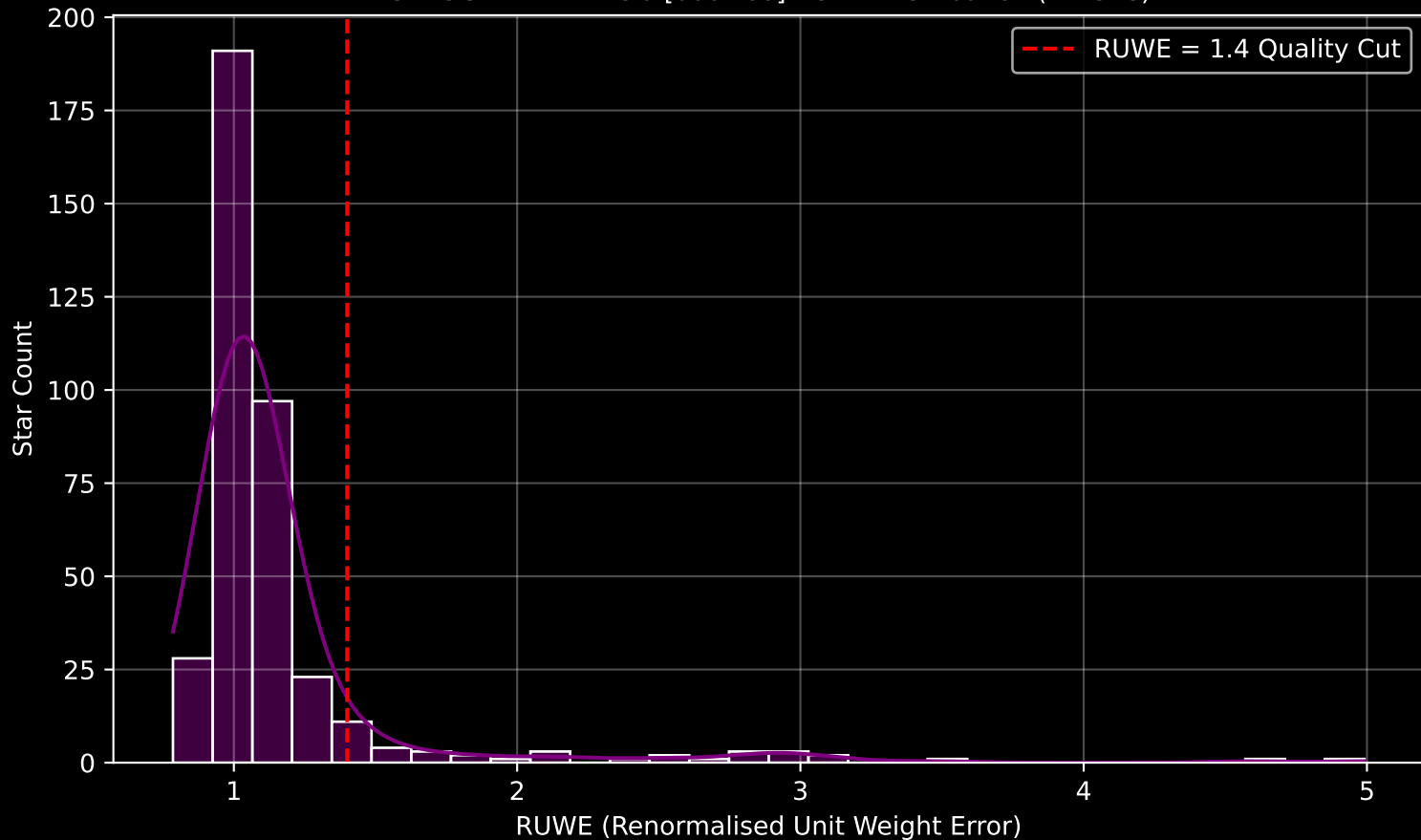
GAPOGEE DR17 Field [000+60] RUWE Distribution (n= 378)
