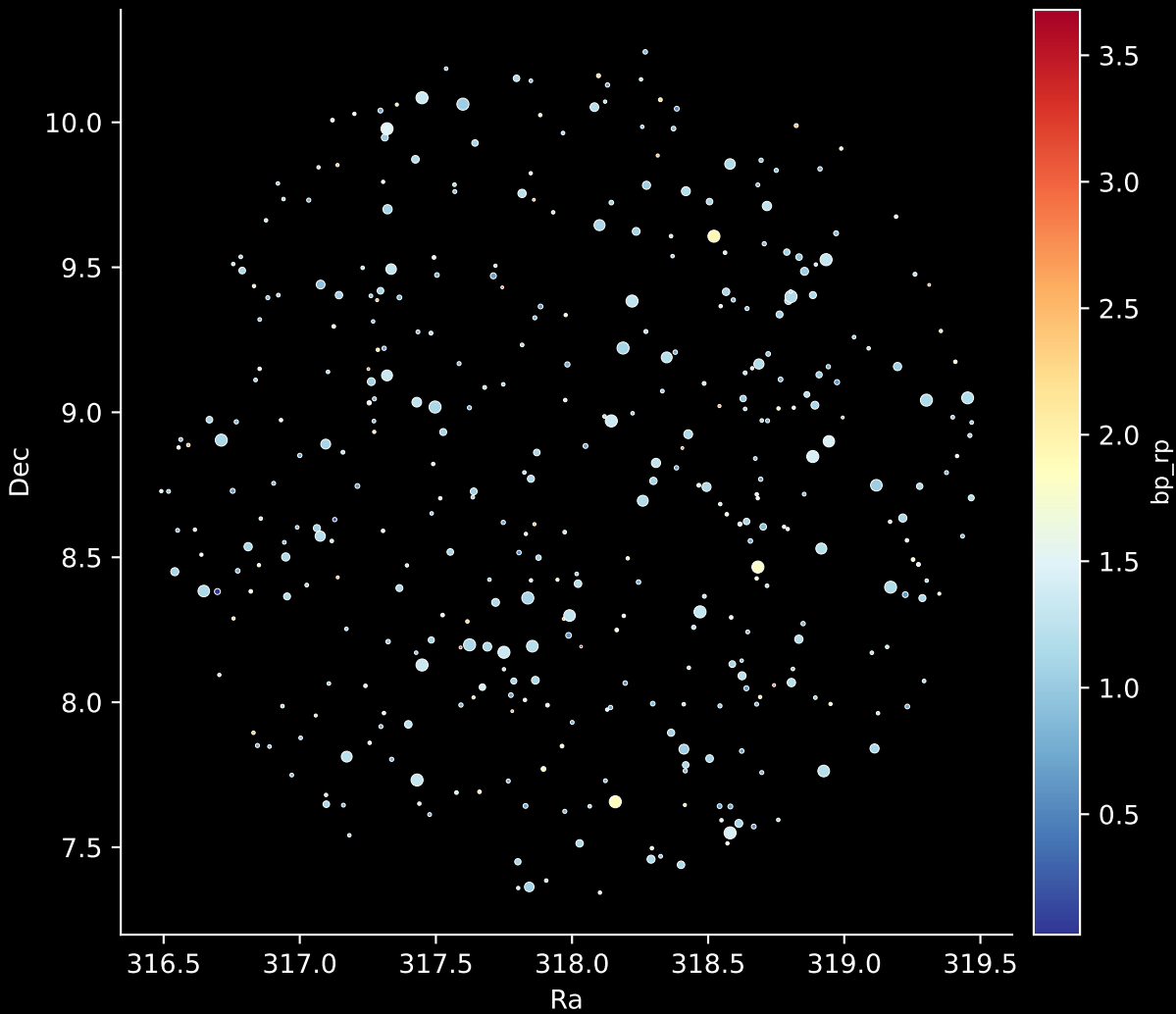
APOGEE DR17 Field: [000+60] Stars: 392
