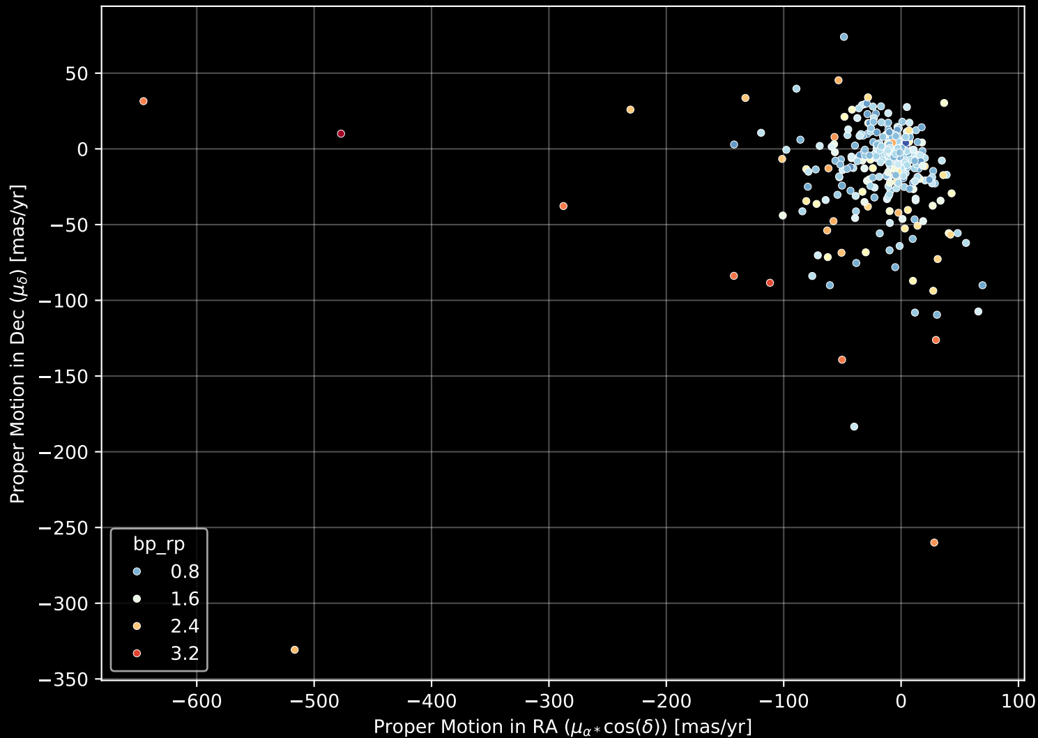
APOGEE DR17 Field: [000+60] Proper Motion Diagram (n= 392)
